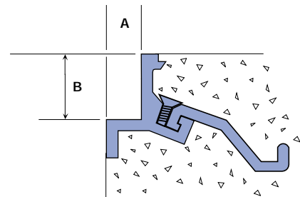
FG25, FG31 & FG37.5 GRATING FRAMES
