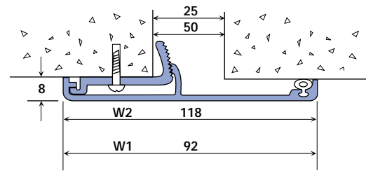
W1 & W2 FLAT WALL/CEILING COVER
