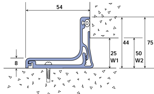
K1 & WX2 CORNER WALL/CEILING COVER
