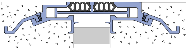
CT2 PLAIN RECESSED
