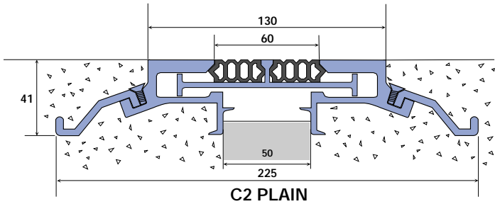
C2 PLAIN
