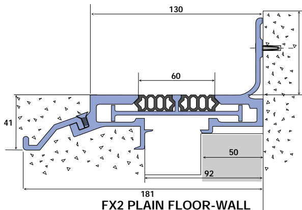
FX2 PLAIN FLOOR-WALL
