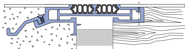
TW2 RECESSED CONCRETE-WOOD TCW2 RECESSED CONCRETE-PLAIN WOOD ONLY (not illustrated)
