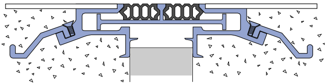
T2 RECESSED
