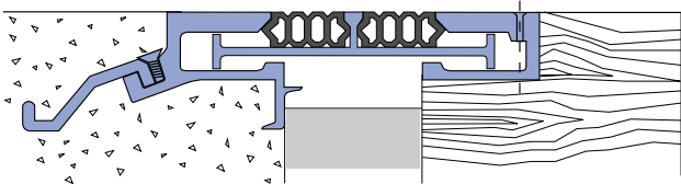
CW2 PLAIN CONCRETE-WOOD CTW2 PLAIN CONCRETE-RECESSED WOOD ONLY (not illustrated)
